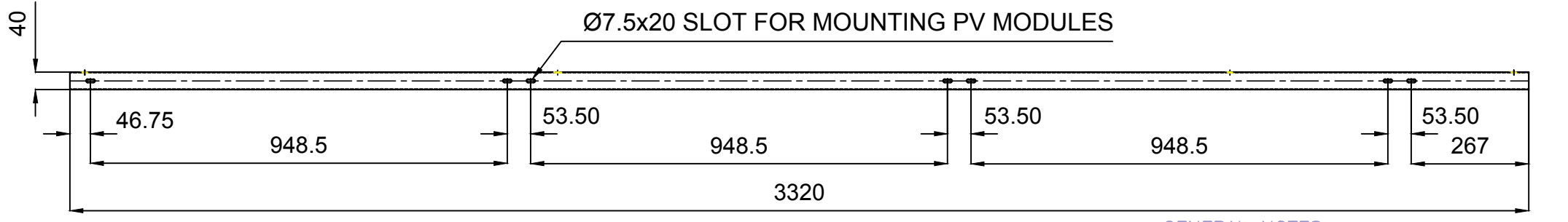
TOP VIEW
