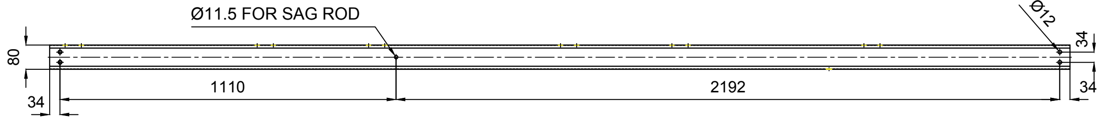
FRONT VIEW
