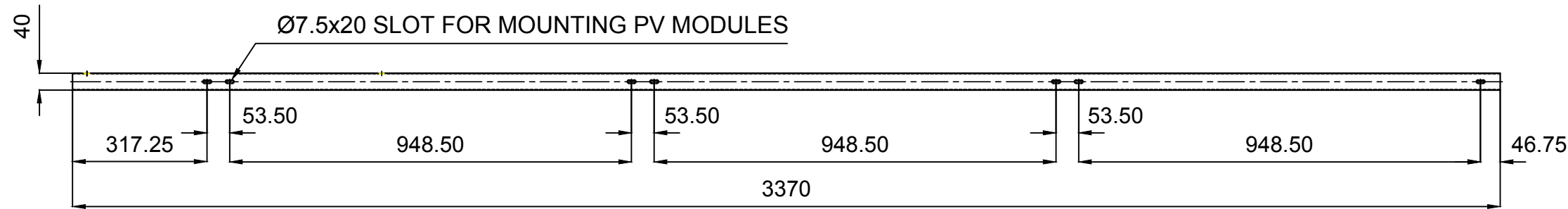
FRONT VIEW
