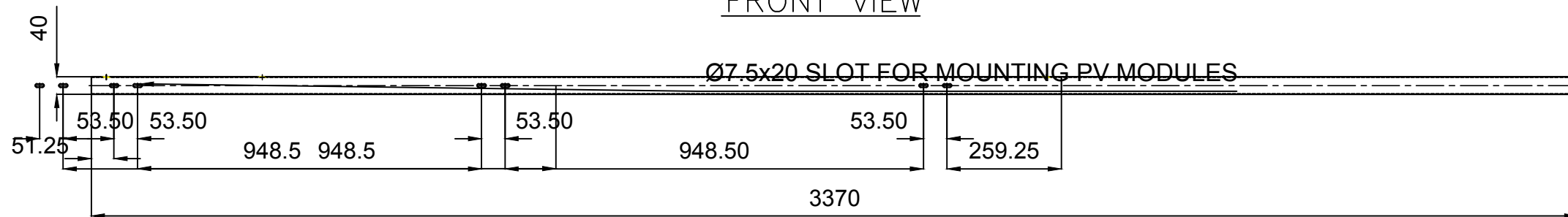
FRONT VIEW
